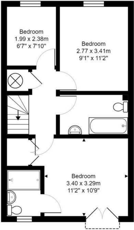
First Floor Area: 41.8 m 2 ... 450 ft 2
