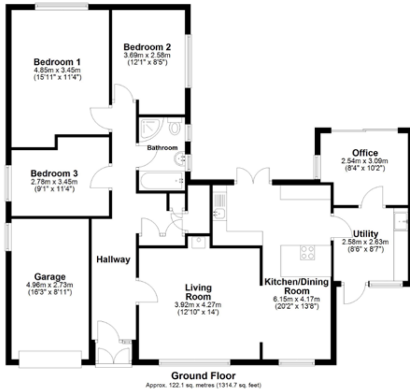
Ground Floor Approx. 122.1 sq. metres (1314.7 sq. feet)
