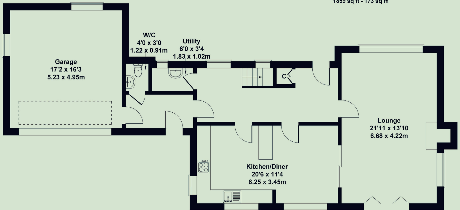
GROUND FLOOR
