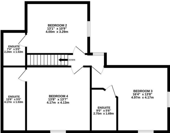
1ST FLOOR 700 sq.ft. (65.0 sq.m.) approx.
