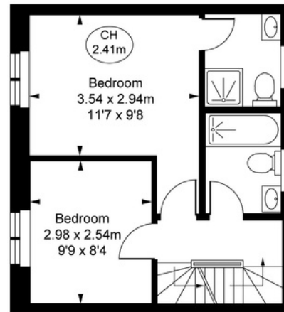
First Floor Approximate Gross Internal Area 31.81 sq m / 342 sq ft
