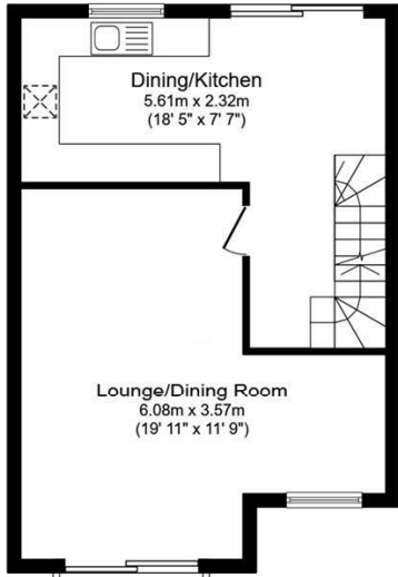
First Floor Floor area 46.3 sq.m. (499 sq.ft.)
